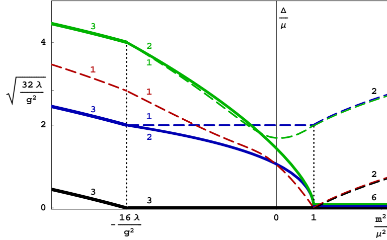
Fig. 1. The energy gaps \Delta of excitations in the model with global U(1)_Y symmetry. The degeneracy factor is specified at each gap line.
