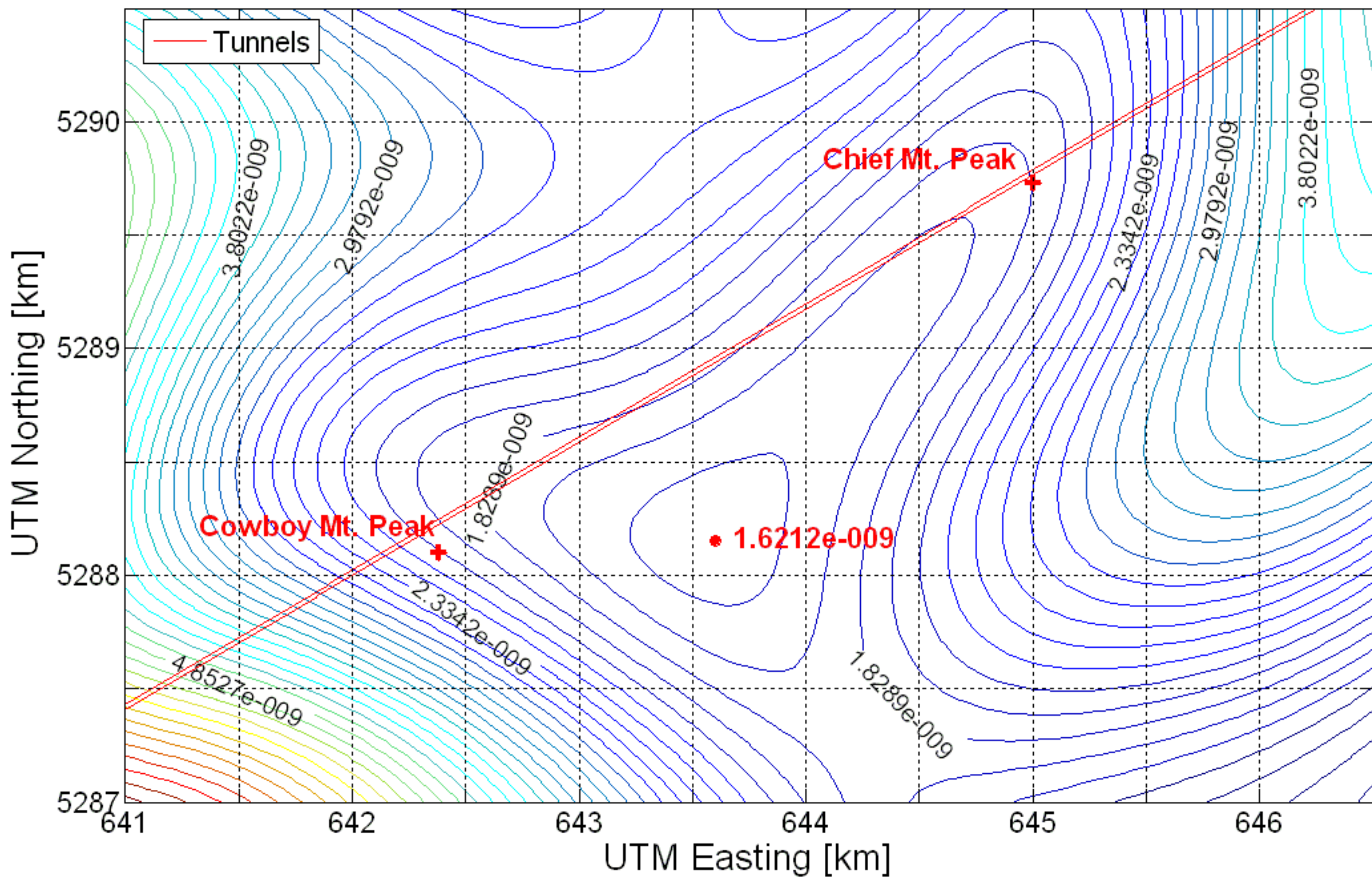
Total \mu Flux [ \text{cm}^{-2} \text{s}^{-1} ] Contours (5% Intervals) at -320[m] Elevation, Pioneer Tunnel
