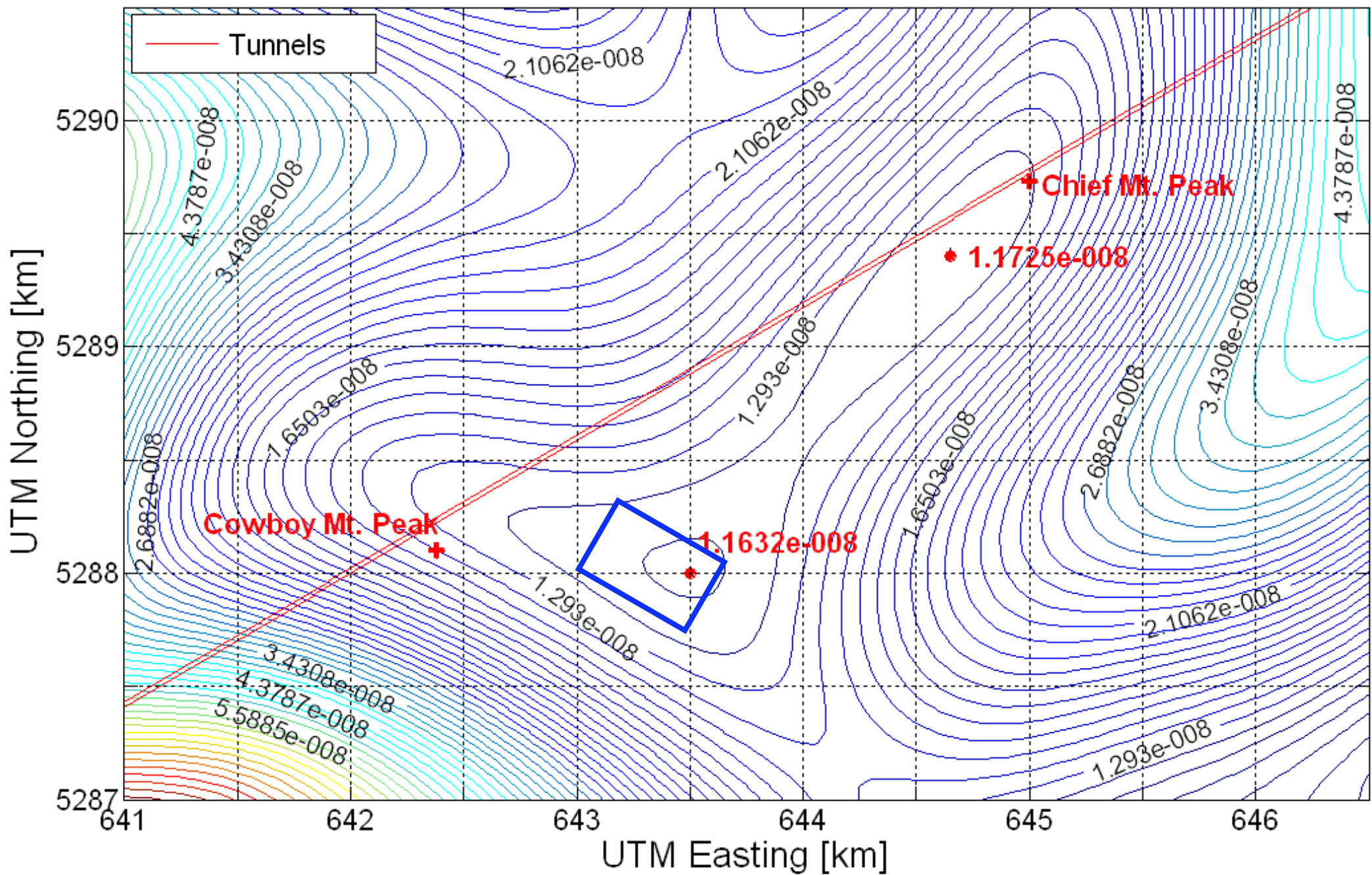
Total \mu Flux [ \text{cm}^{-2} \text{s}^{-1} ] Contours (5% Intervals) at 177[m] Elevation, Pioneer Tunnel
