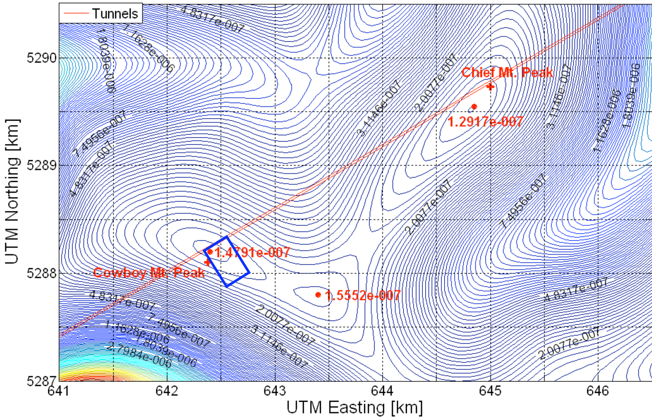
Total \mu Flux [ \text{cm}^{-2} \text{s}^{-1} ] Contours (5% Intervals) at 743[m] Elevation, Pioneer Tunnel
