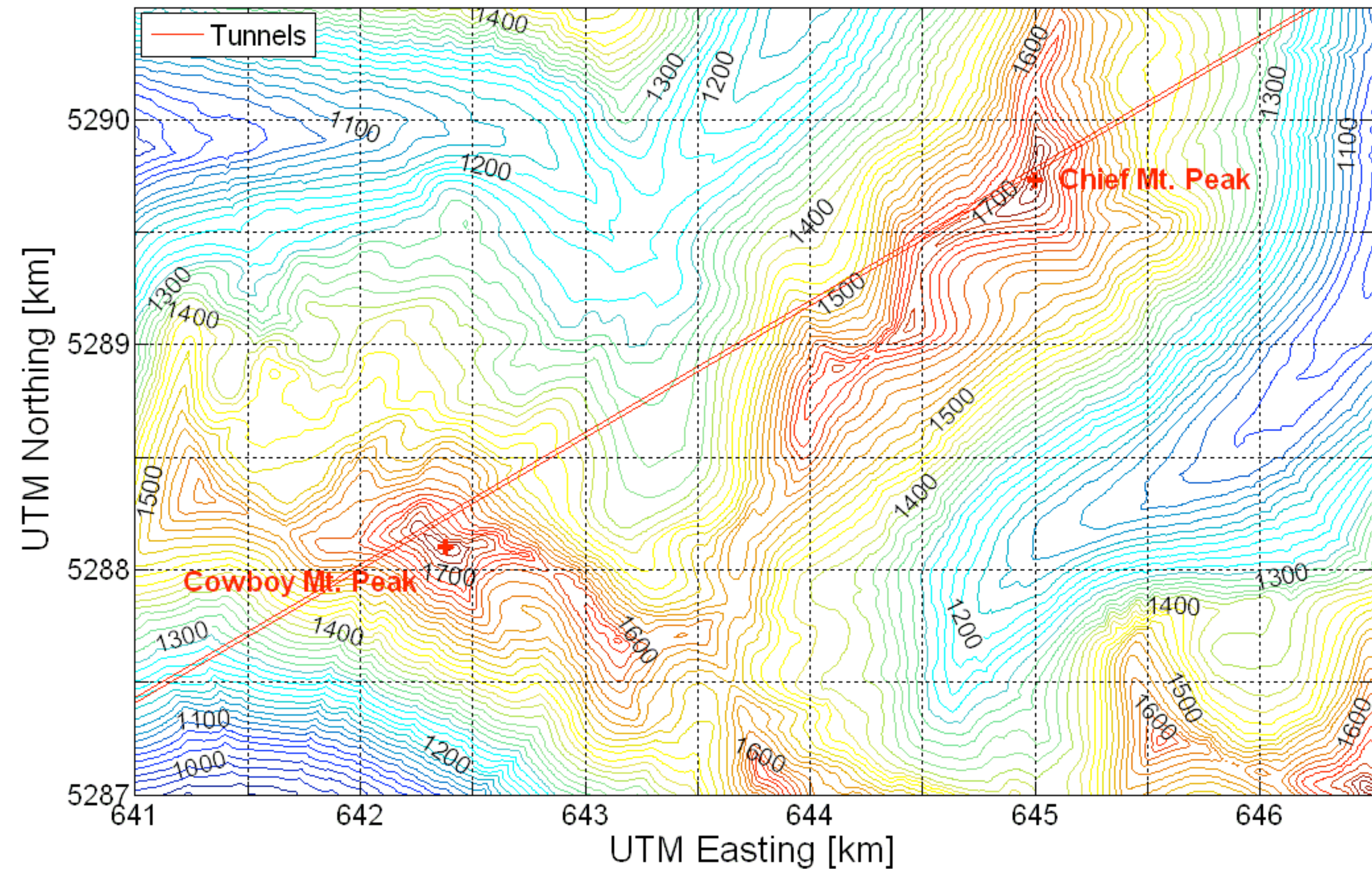
Pioneer Tunnel Elevation Contours, 20[m] Resolution
